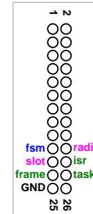
OpenWSN debugpins
