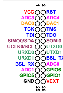
pin functions
