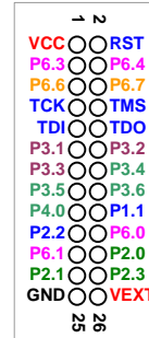
pin names
